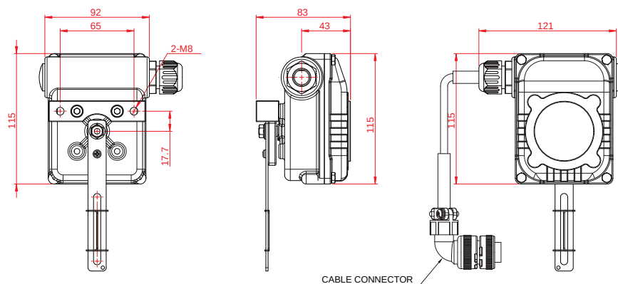
< Linear Type Remote Position Unit >
