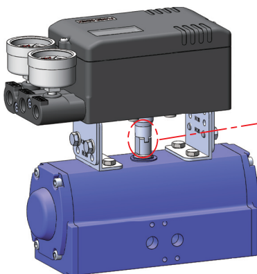
NAMUR Type Mounting ( VDI/VDE 3845, IEC 60534-6-2 )
