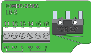
Micro switches 1, 2
