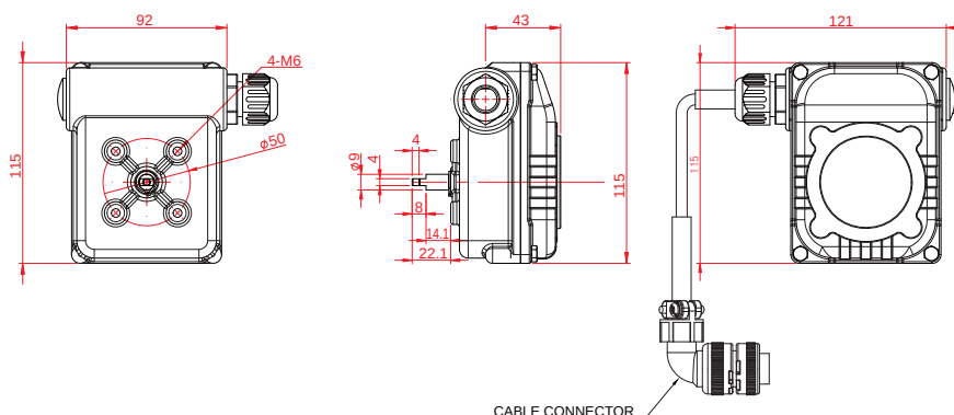
< Rotary Type Remote Position Unit >
